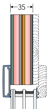
Tipo TM 35 Up 0.86 W/m 2 k Rw 33 dB Kg 18,0 m 2
